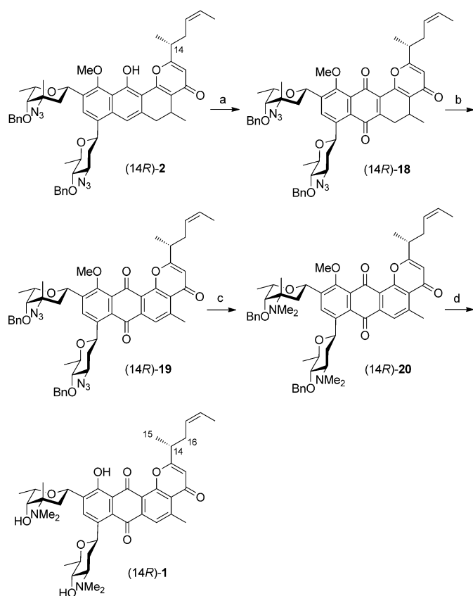
Scheme 5. Completion of the total synthesis of (14R)-1: a) PhI-(OCOCF 3 ) 2 , H 2 O, MeCN, 0°C, 1 h; b) DBU, MeCN, 0°C, 30 min, then air, room temperature, 1 h (67% from (14R)-2); c) PMe 3 , CH 2 Cl 2 , room temperature, 4 h; 37% aqueous HCHO, NaBH 3 CN, AcOH, MeCN, 0°C→RT, 2 h (65%); d) BBr 3 , CH 2 Cl 2 , −90°C, 1 h (62%). DBU = 1,8-diazabicyclo[5.4.0]undec-7-ene.
