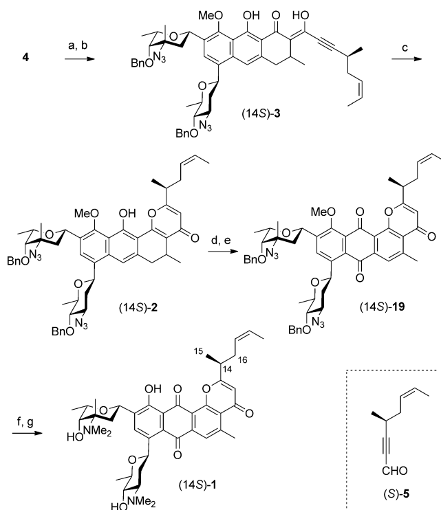
Scheme 6. Synthesis of (14S)-1: a) LDA, THF, −78→0°C, 1 h, then ( S )-5, −78°C, 1 h (90%); b) IBX, DMSO, CH 2 Cl 2 , room temperature, 3 h (84%); c) K 2 CO 3 , MeOH, room temperature, 6 h (89%); d) PhI-(OCOCF 3 ) 2 , H 2 O, MeCN, 0°C, 1 h; e) DBU, MeCN, 0°C, 30 min, then air, room temperature, 1 h (59% from 3); f) PMe 3 , CH 2 Cl 2 , room temperature, 4 h; 37% aqueous HCHO, NaBH 3 CN, AcOH, MeCN, 0°C→RT, 2 h (64%); g) BBr 3 , CH 2 Cl 2 , −90°C, 1 h (73%).
