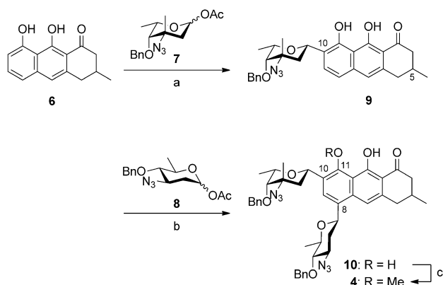
Scheme 2. Bis- C -glycosylation of tricyclic 6 : a) \text{Sc}(\text{OTf})_3 (30 mol %), Drierite, \text{ClCH}_2\text{CH}_2\text{Cl} , -30 \rightarrow -10^\circ\text{C} , 3 h (82 %); b) \text{Sc}(\text{OTf})_3 (50 mol %), Drierite, \text{ClCH}_2\text{CH}_2\text{Cl} , -30 \rightarrow 28^\circ\text{C} , 12 h (96 %); c) \text{CH}_3\text{I} , NaH, TBAI, DMF, 0^\circ\text{C} , 5 h (99 %). DMF = N,N -dimethylformamide, TBAI = tetrabutylammonium iodide.
