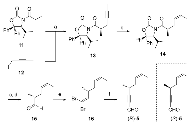
Scheme 3. Synthesis of the enantiomeric alkynals ( R )- and ( S )- 5 : a) LDA, 12 , THF, -78^\circ\text{C} \rightarrow \text{RT} , 10 h (95 %, d.r. > 99:1); b) \text{H}_2 (balloon), Lindlar catalyst, quinoline, EtOAc, room temperature, 5 h (93 %); c) \text{LiAlH}_4 , \text{Et}_2\text{O} , 0^\circ\text{C} , 1 h; d) TPAP (5 mol %), NMO, MS (4 Å), \text{CH}_2\text{Cl}_2 , 0^\circ\text{C} \rightarrow \text{RT} , 2 h; e) \text{CBr}_4 , \text{PPh}_3 , Zn, \text{CH}_2\text{Cl}_2 , room temperature, 3 h (84 % from 14 ); f) n\text{BuLi} , THF, -78 \rightarrow -20^\circ\text{C} ; DMF, -78 \rightarrow 0^\circ\text{C} , 2 h (80 %). LDA = lithium diisopropylamide, TPAP = tetrapropylammonium per-ruthenate, NMO = 4-methylmorpholine N -oxide, MS = molecular sieves.
